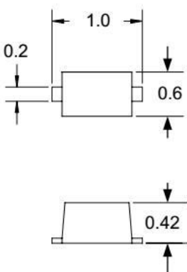
Dimensions (mm)
