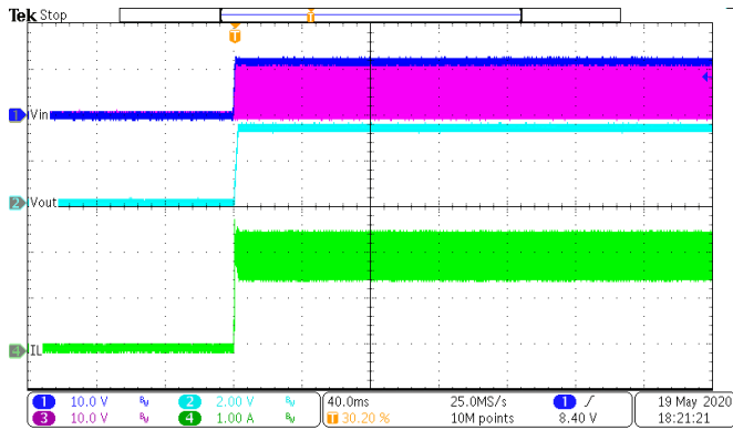
Figure 20. Power up
