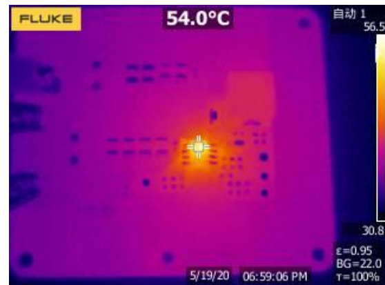
Figure 25. Thermal, 3.3Vout/2A
