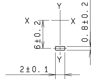
LOCATING LUG DETAIL シャーシ止め詳細図
