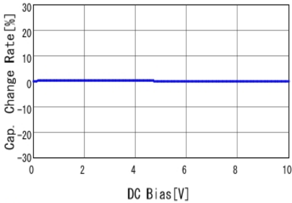
■ GRM21B7U1A104JA01 C-DC bias capchange, 25.0degC, AC1V
