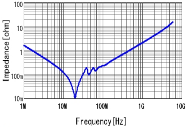
■ GRM21B7U1A104JA01 |Z| DCOV, 25degC
