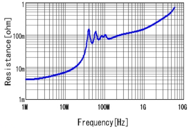
■ GRM21B7U1A104JA01 R DCOV, 25degC
