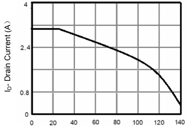
Figure 4 Drain Current
