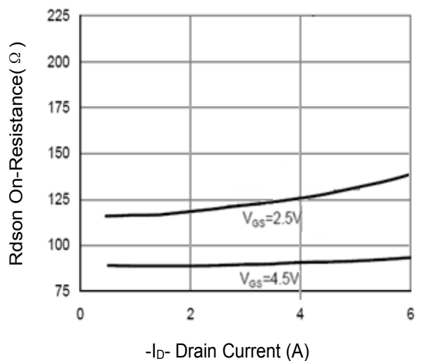
Figure 6 Drain-Source On-Resistance
