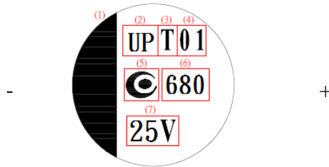
Figure 3 Marking
