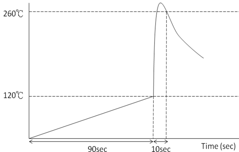
Figure 7 Flow Curve
