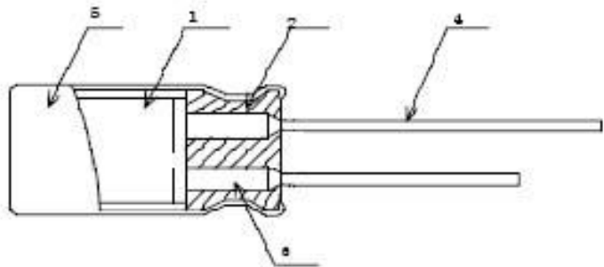
Fig. 1 Cross-section view
