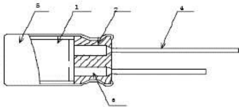
Fig. 1 Cross-section view
