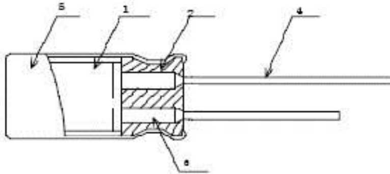
Fig. 1 Cross-section view
