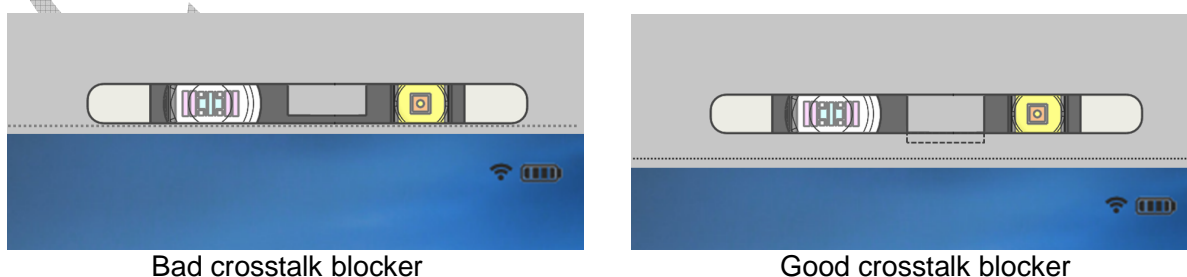
Figure 3 – Blocker in slit to block crosstalk
