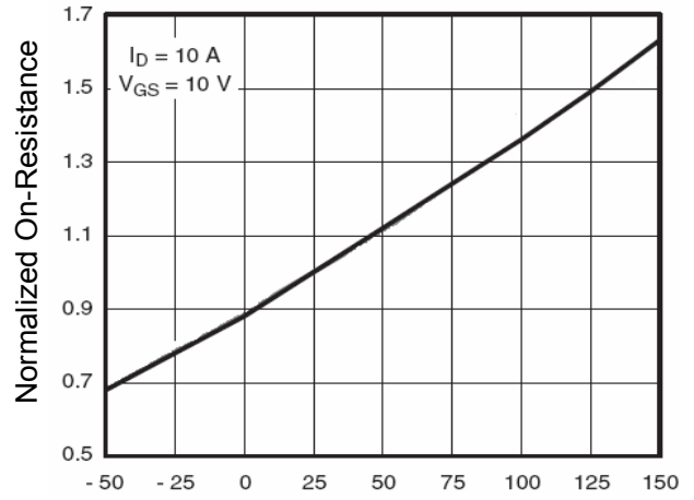
T_J -Junction Temperature( ^\circ\text{C} ) Figure 8 Drain-Source On-Resistance
