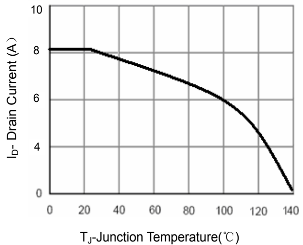
Figure 4 Drain Current
