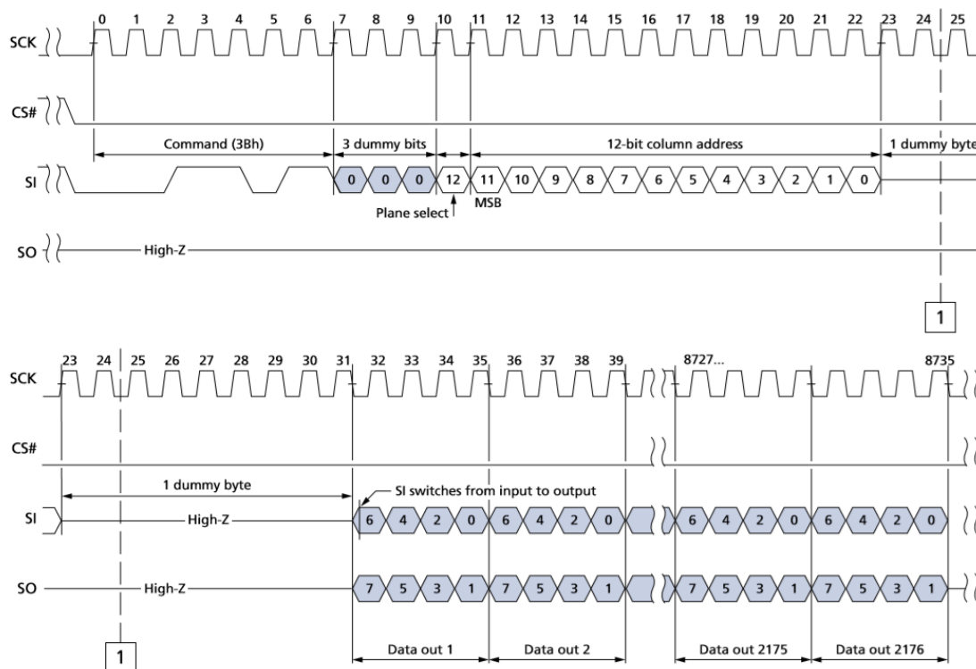
Figure8. READ FROM CACHE x2
