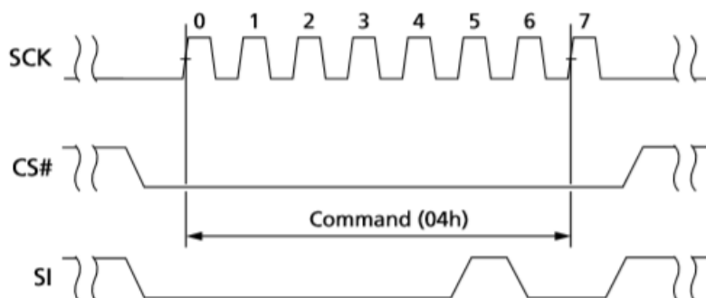
Figure5. WRITE DISABLE (04h) Timing
