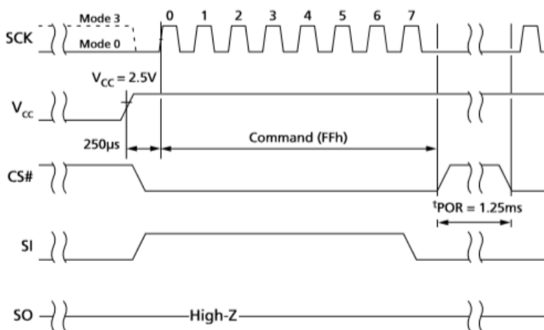
Figure25. SPI Power-Up Timing
