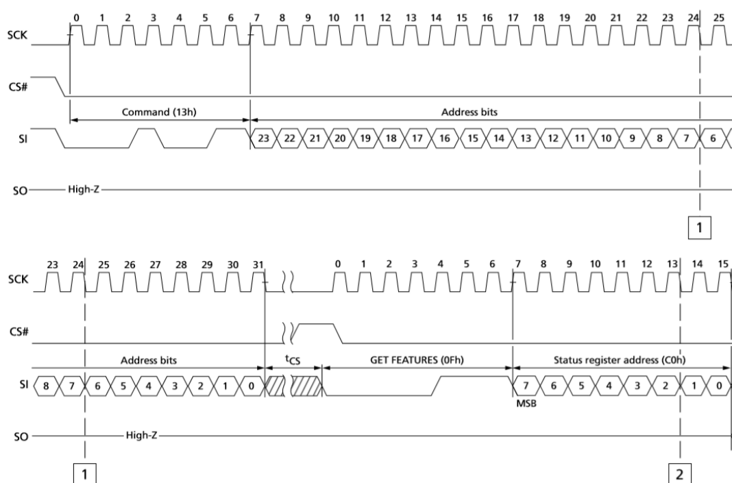
Figure6. PAGE READ (13h) Timing
