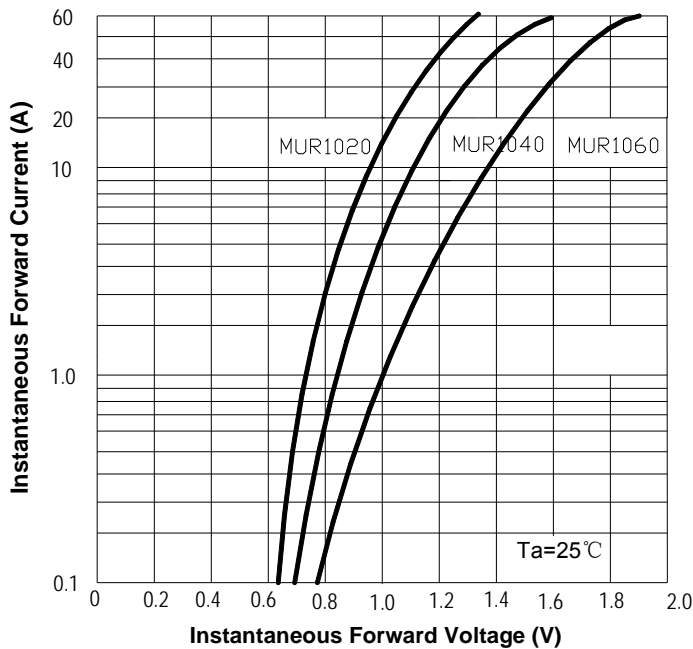
FIG3: Forward Voltage
