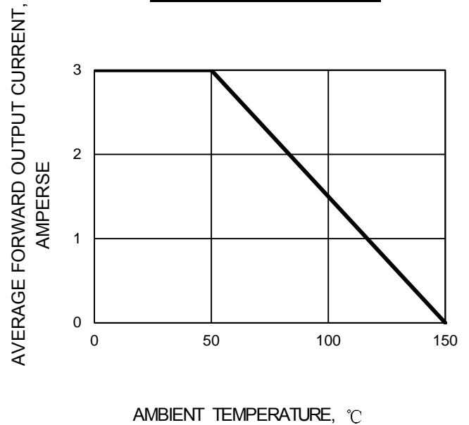
FIG.2 – FORWARD DERATING CURVE OUTPUT RECTIFIED CURRENT
