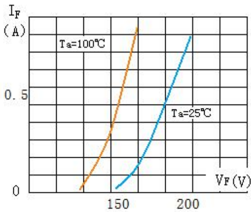
正向特性曲 ( 2CL150KV/0.5A ) Forward Characteristics
