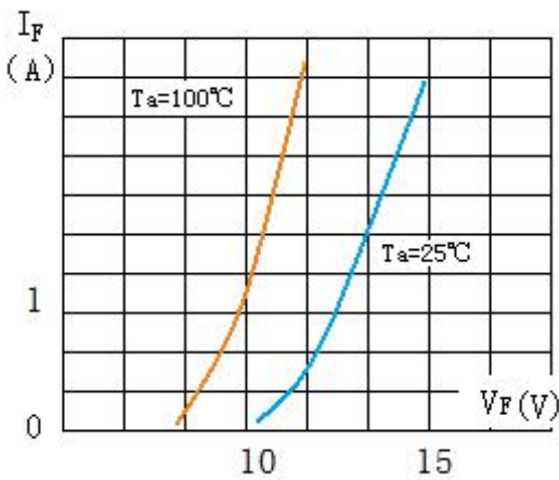
正向特性曲 ( 2CL10KV/1A ) Forward Characteristics
