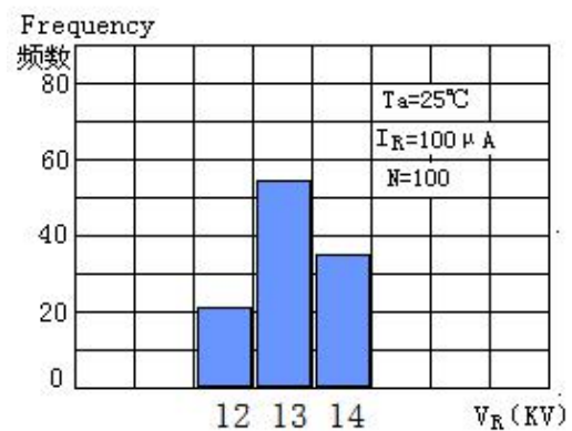
反向雪崩电压分布 ( 2CL10KV/1A ) Avalanche Breakdown Voltage Distribution
