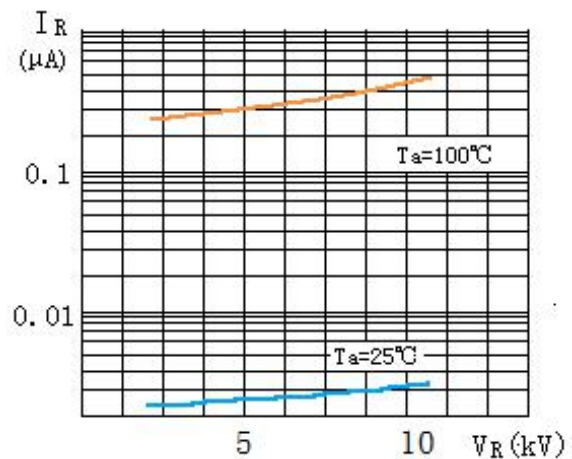
反向特性曲线 ( 2CL10KV/1A ) Reverse Characteristics
