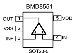
Figure 1. Pin Assignment Diagram
