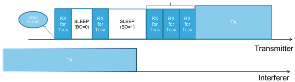
Figure 26. CSMA with non-persistent mode if channel becomes free (timeline)
