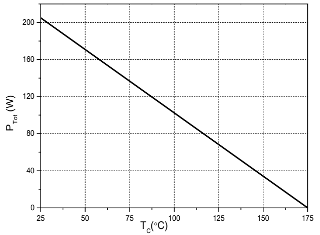
Figure 6. Power Derating
