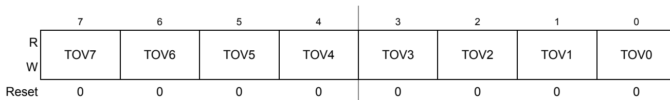
Figure 23-13. Timer Toggle On Overflow Register 1 (TTOV)
