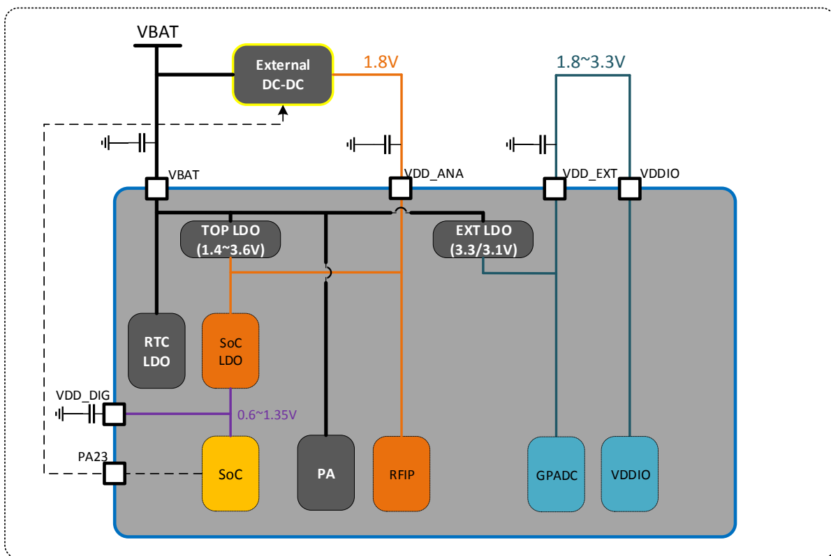
Figure 2-1 Power Architecture
