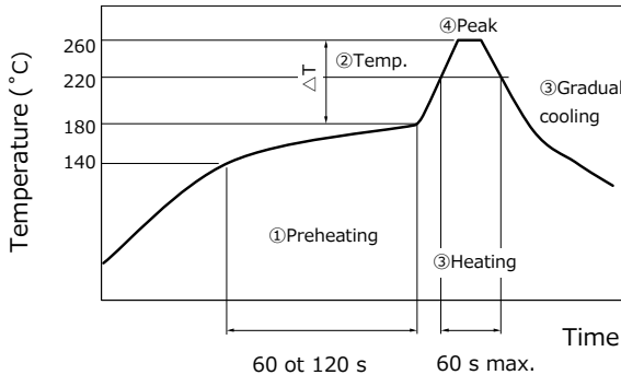
Recommended profile of Reflow Soldering (Ex.)
