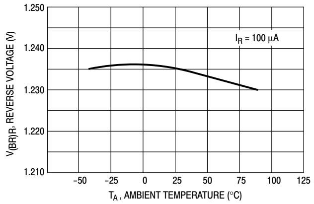
Figure 5. Temperature Drift
