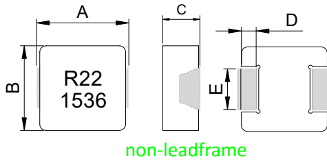
leadframe
