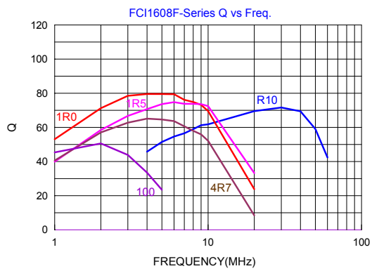
■ Q-Frequency Characteristics
