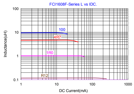
■ Inductance-Current
