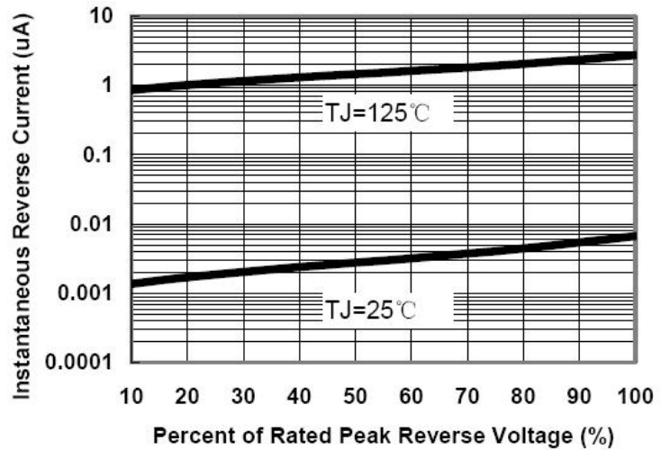
Fig.2-Typical Reverse Characteristics
