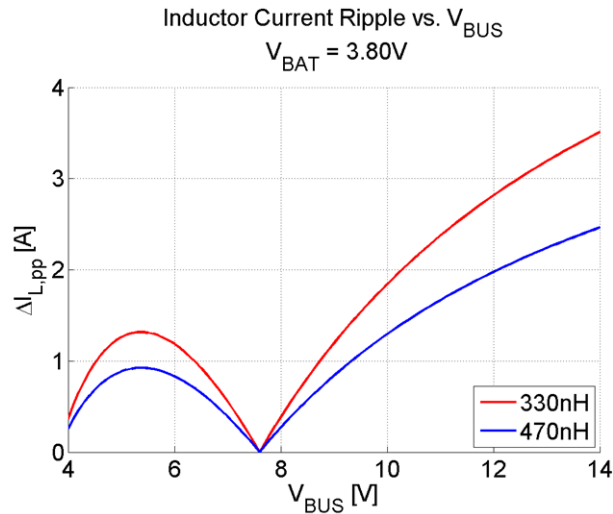
Figure 46. Inductor Current Ripple as function of V BUS with Fixed V BAT
