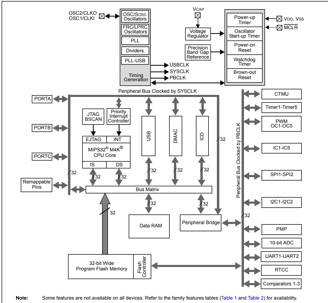
FIGURE 1-1: BLOCK DIAGRAM
