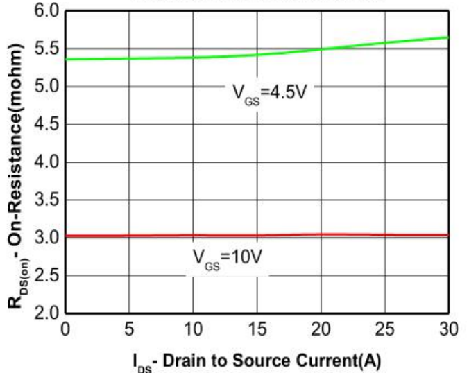
Figure 6. R_DS(on)-Drain Current
