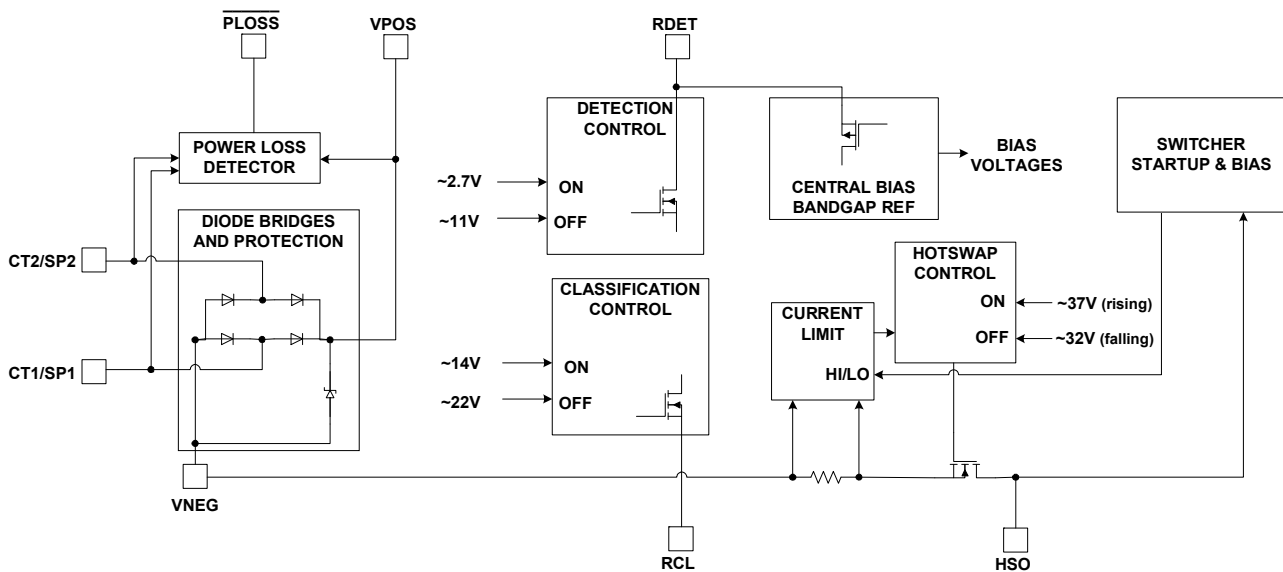
Figure 3. Input Lineside and Hotswap Block Diagram
