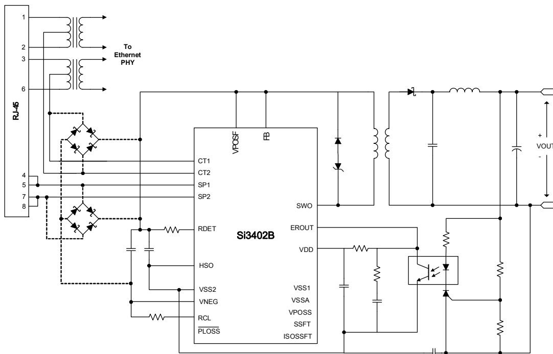
Figure 2. Schematic—Isolated Flyback Topology
