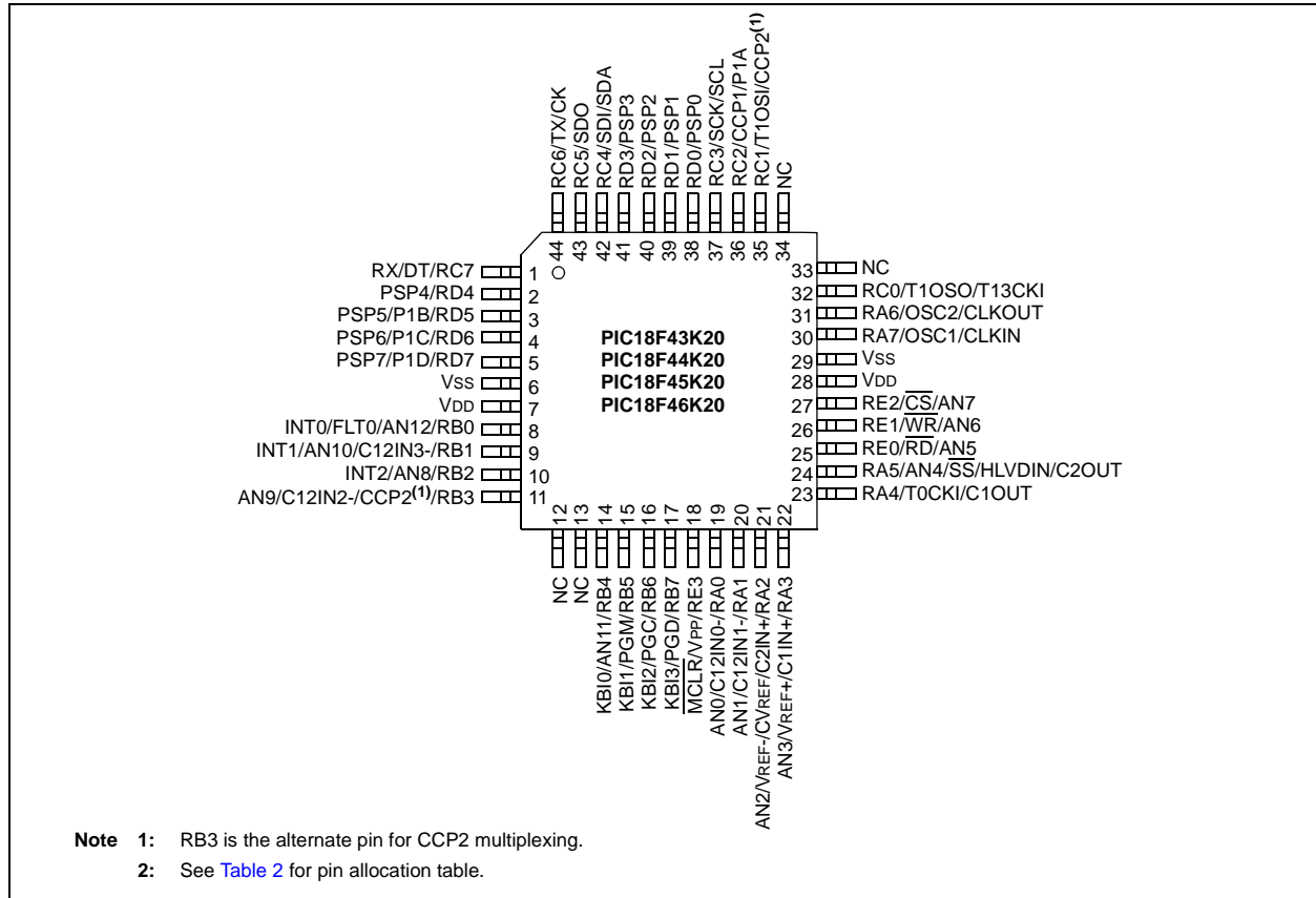
FIGURE 6: 44-PIN TQFP
