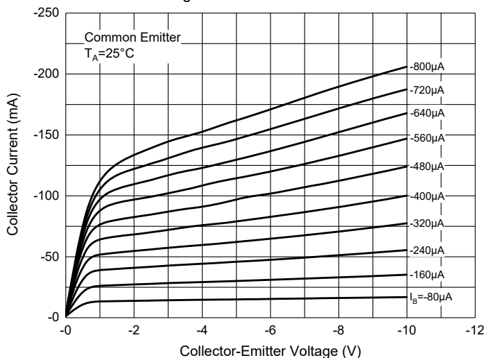
Fig. 7 - Static Characteristics
