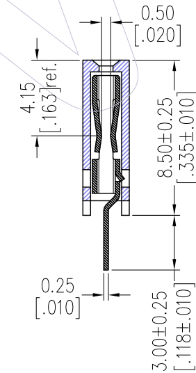
Section X-X
