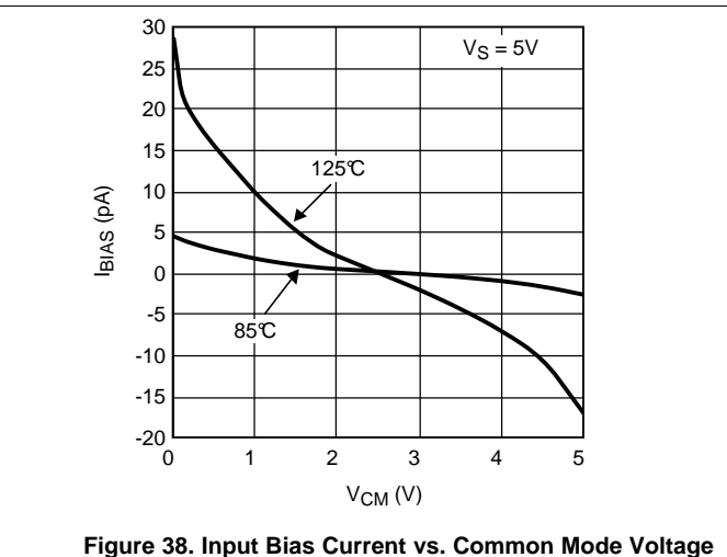
Figure 38. Input Bias Current vs. Common Mode Voltage
