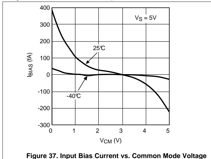
Figure 37. Input Bias Current vs. Common Mode Voltage
