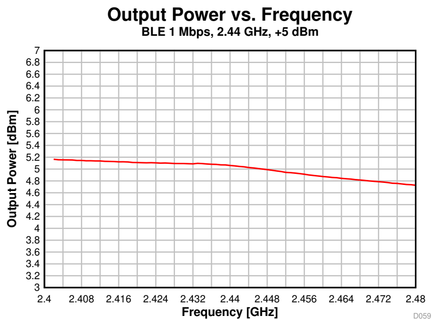
Figure 5-22. Output Power vs. Frequency (BLE 1 Mbps, 2.44 GHz, +5 dBm)
