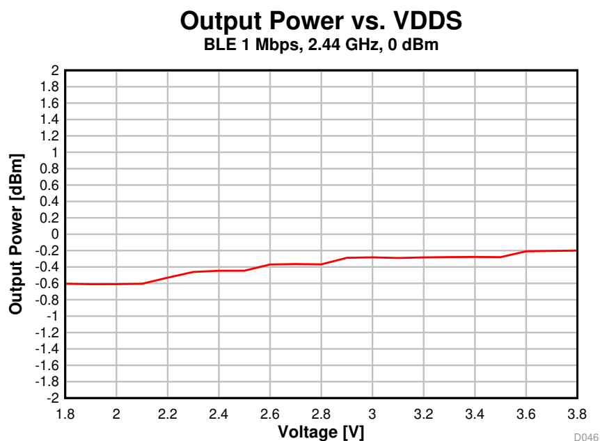
Figure 5-19. Output Power vs. Supply Voltage (VDDS) (BLE 1 Mbps, 2.44 GHz)
