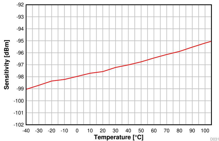
Figure 5-12. Sensitivity vs. Temperature (BLE 1 Mbps, 2.44 GHz)
