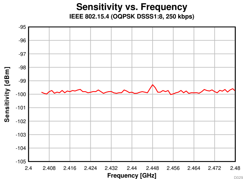
Figure 5-11. Sensitivity vs. Frequency (250 kbps, 2.44 GHz)
