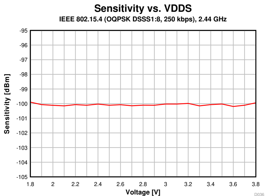
Figure 5-16. Sensitivity vs. Supply Voltage (VDDS) (250 kbps, 2.44 GHz)
