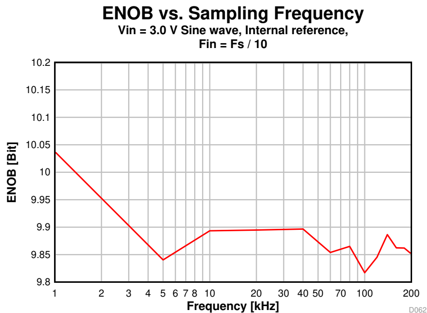
Figure 5-24. ENOB vs. Sampling Frequency
