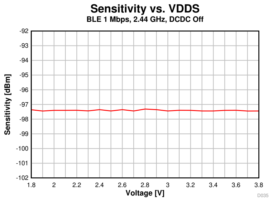
Figure 5-15. Sensitivity vs. Supply Voltage (VDD5) (BLE 1 Mbps, 2.44 GHz, DCDC Off)
