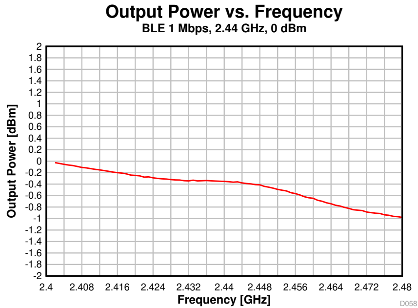
Figure 5-21. Output Power vs. Frequency (BLE 1 Mbps, 2.44 GHz)
