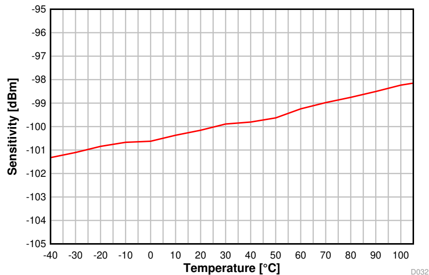
Figure 5-13. Sensitivity vs. Temperature (250 kbps, 2.44 GHz)
