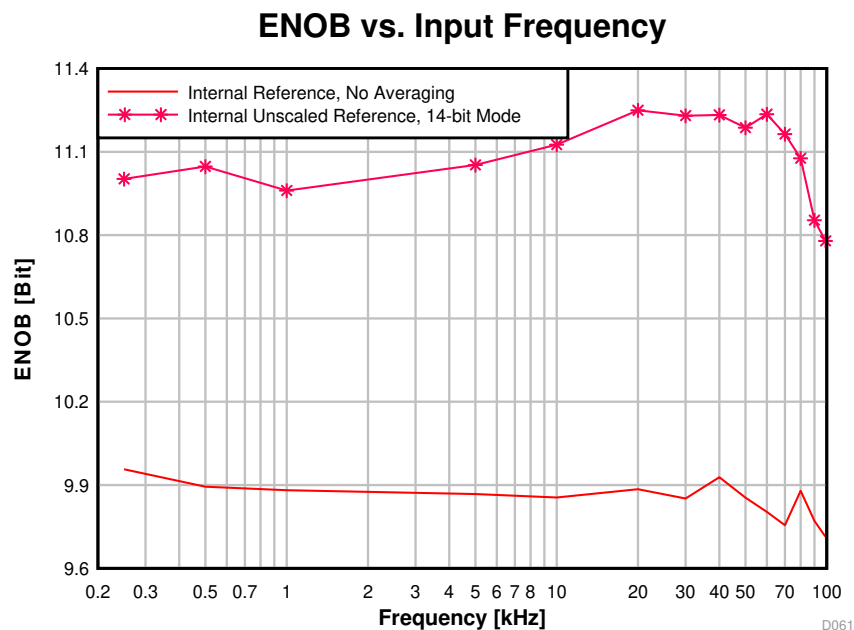
Figure 5-23. ENOB vs. Input Frequency
