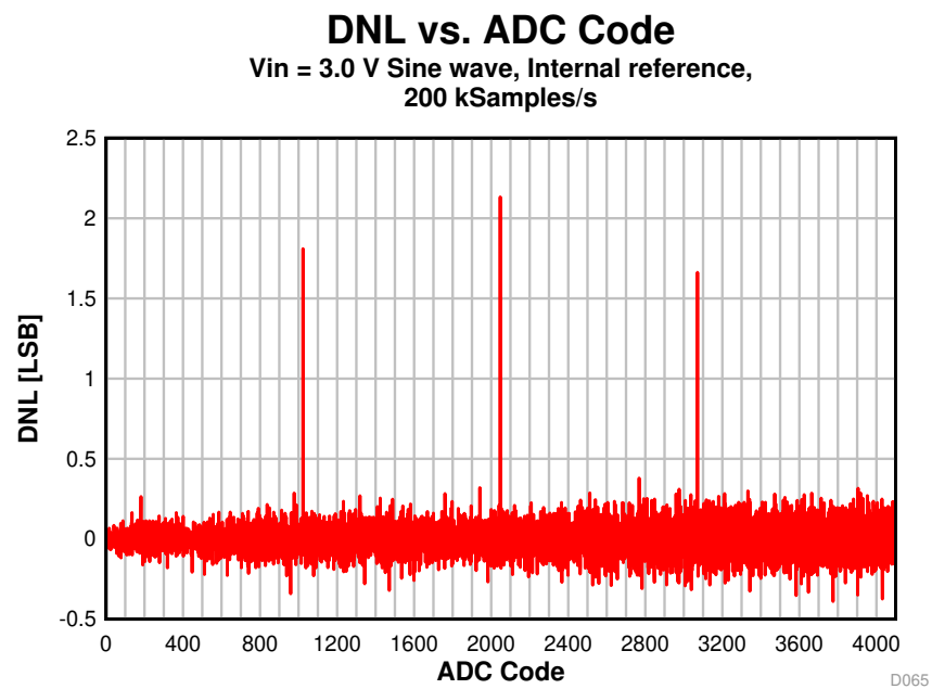
Figure 5-26. DNL vs. ADC Code
