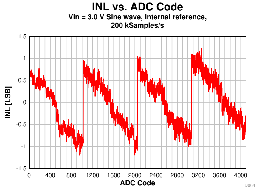
Figure 5-25. INL vs. ADC Code
