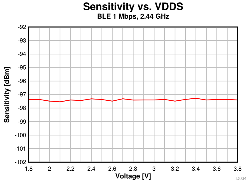
Figure 5-14. Sensitivity vs. Supply Voltage (VDD5) (BLE 1 Mbps, 2.44 GHz)
