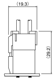
Inner-housing lock
