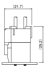
Outer-housing lock
