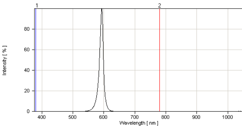
Fig.1 Super Yellow Relative Intensity vs. Wavelength
