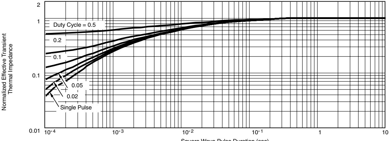
Square Wave Pulse Duration (sec) Normalized Thermal Transient Impedance, Junction-to-Case
