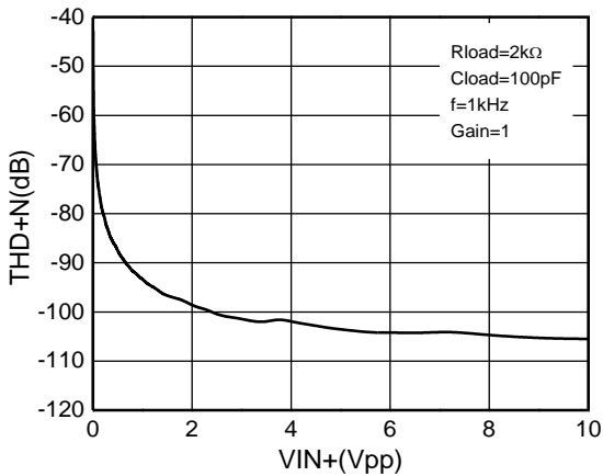
THD+N vs. V_{IN+}
