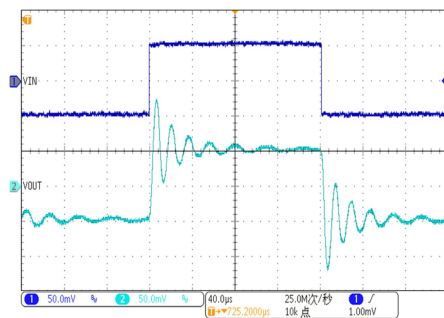
Over Shoot Voltage, C_{\text{load}}=47\text{nF} , R_{\text{FB}}=10\text{k}\Omega , Gain=+1
