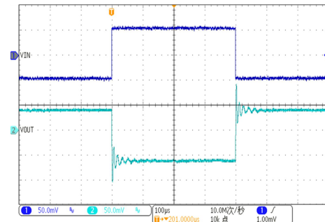
Over Shoot Voltage, C_{\text{load}}=47\text{nF} , R_{\text{load}}=40\text{k}\Omega , Gain=-1
