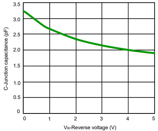
Fig 6. Capacitance vs. Reverse voltage
