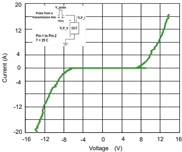
Fig 5. TLP Measurement
