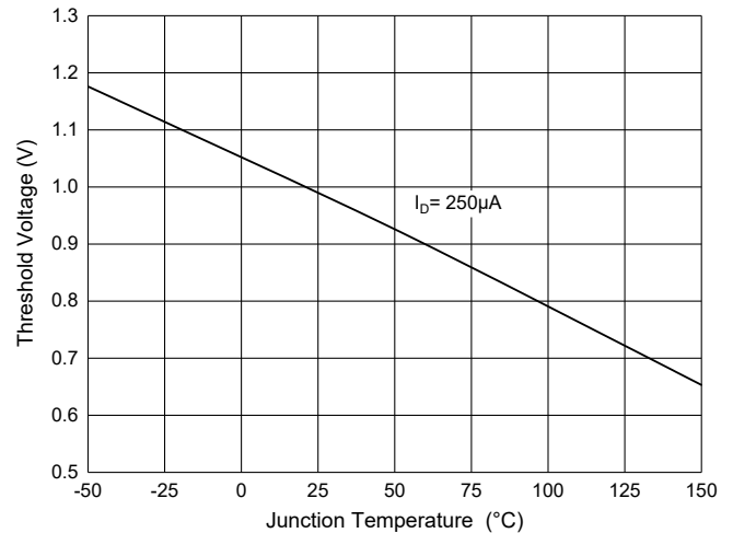
Fig. 6 - Threshold Voltage
