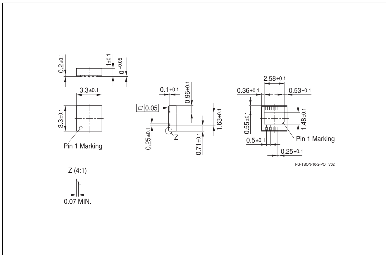
Figure 6 PG-TSON-10
