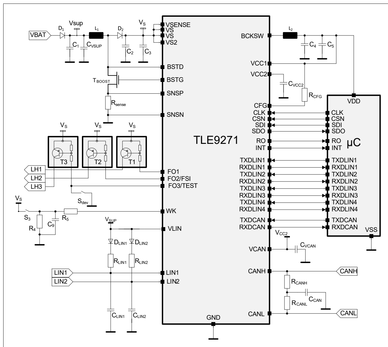
Figure 50 Application Diagram
