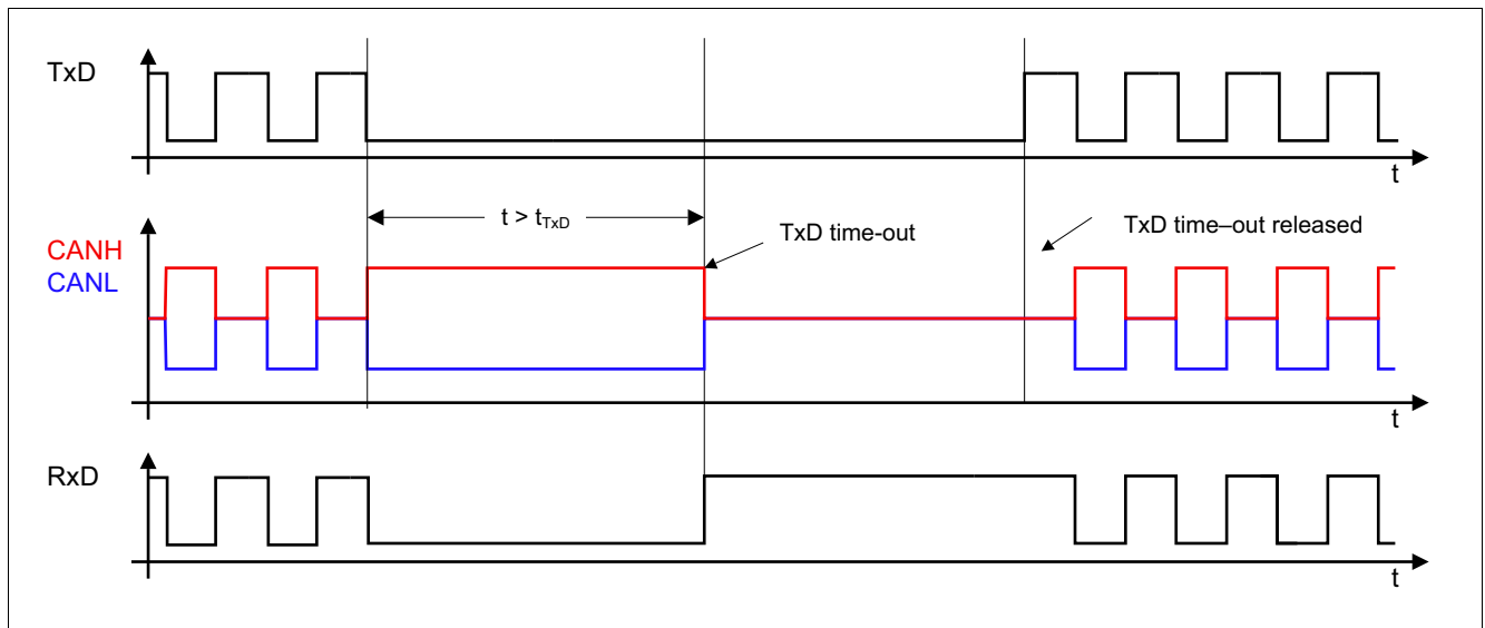
Figure 11 TxD time-out function
