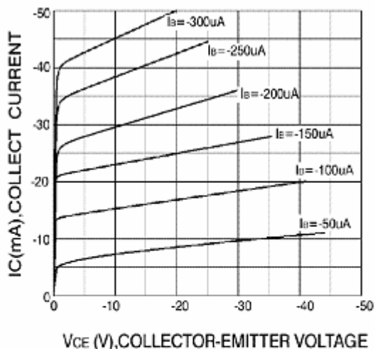
Static Characteristic
