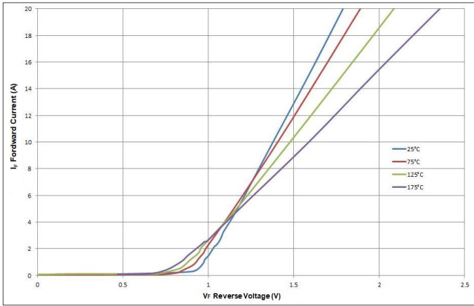
Fig. 1 Forward Characteristics
