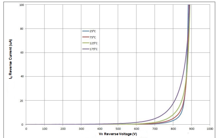
Fig. 2 Reverse Characteristics
